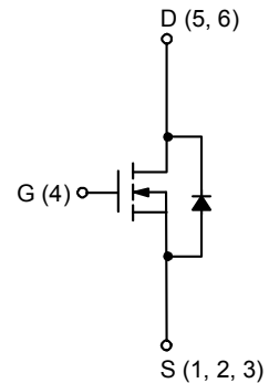
N-Channel MOSFET
