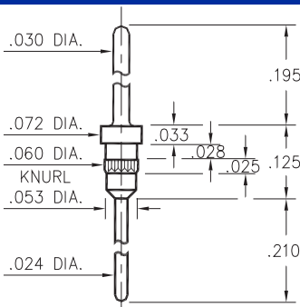
5005-0-00-XX-00-00-03-0 Press-fit in .057 mounting hole
