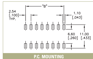
P.C. MOUNTING
