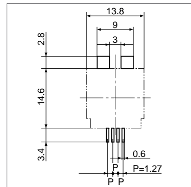
LAND LAYOUT
