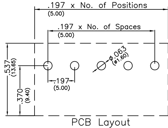
Application View
