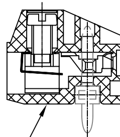
Application View
