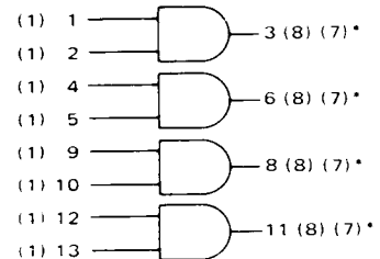
MC1806/MC1906 MC1807/MC1907 Quad 2-Input AND Gate
