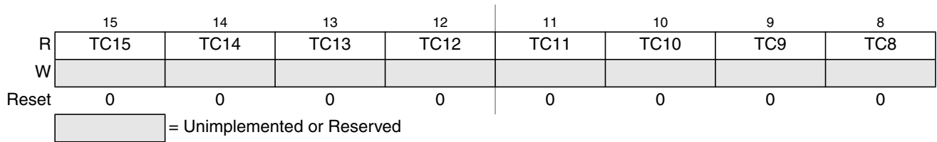
Figure 14-62. Timer Input Capture Holding Register 2 High (TC2H)
