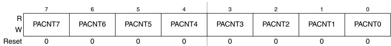
Figure 14-38. Pulse Accumulators Count Register 2 (PACN2)
