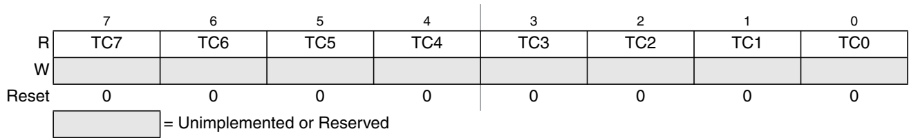
Figure 14-61. Timer Input Capture Holding Register 1 Low (TC1H)
