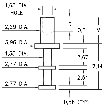
2702-X-00-XX-00-00-07-0 Swage mount in 2,39 hole
