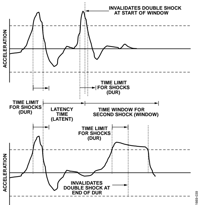
Figure 35. Shock Interrupt Function with Invalid Double Shocks
