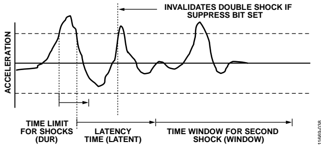
Figure 34. Double Shock Event Invalid Due to High g Event When the Suppress Bit Is Set
