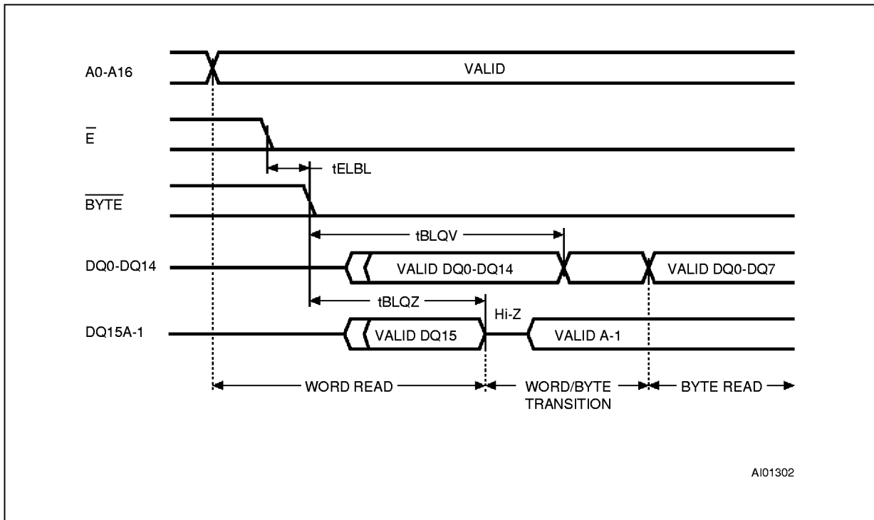
Figure 7. BYTE Mode AC Waveforms, \overline{\text{BYTE}} High to Low
