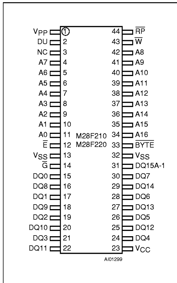
Figure 2B. SO Pin Connections
