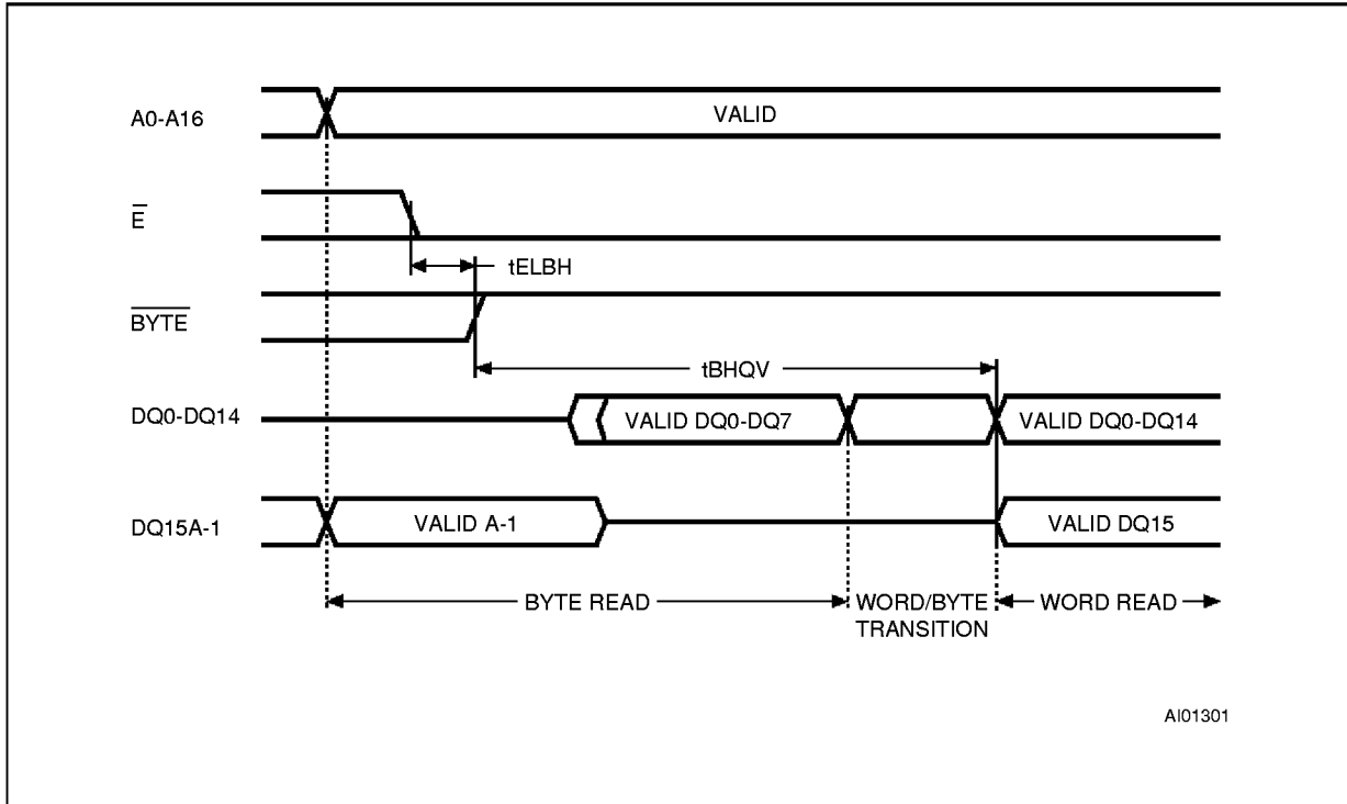
Figure 6. BYTE Mode AC Waveforms, \overline{\text{BYTE}} Low to High
