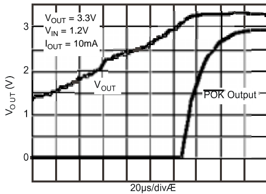
Power Good Output (POK)
