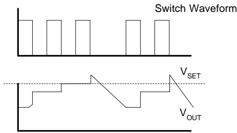
Figure 5: PFM Waveform
