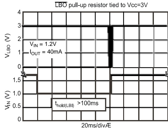
Low Battery Output ( V_{IN} < V_{TH} for Greater than 100ms)
