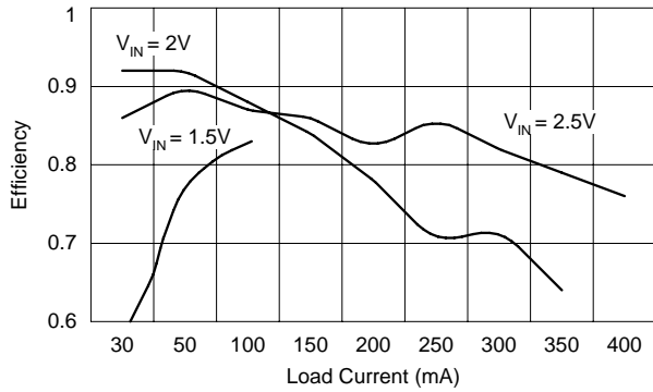
Efficiency (PWM Mode)
