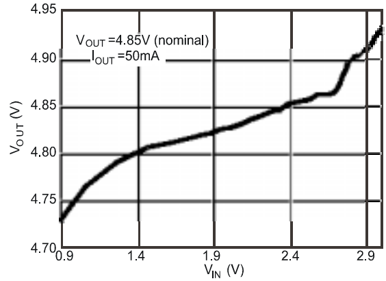
Line Regulation
