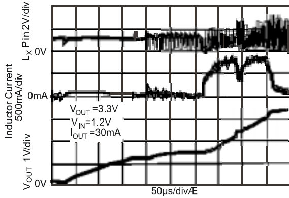
Start-up (PWM Mode)
