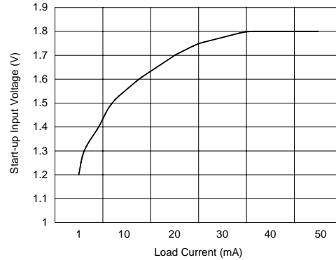
Start-up Input Voltage vs Output current i(PFM Mode)
