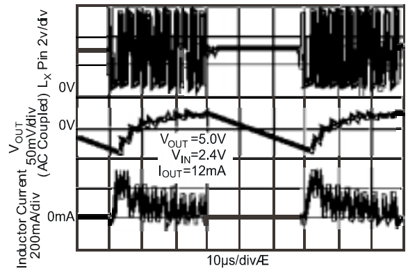
Load Switching Waveforms (PFM Mode)
