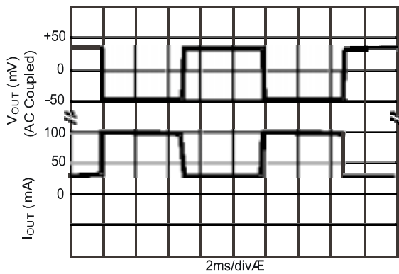
Load Transient Response (25 mA to 100 mA Load Step)
