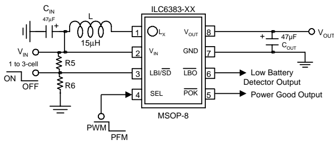
Figure 1: ILC6383CIR-XX
