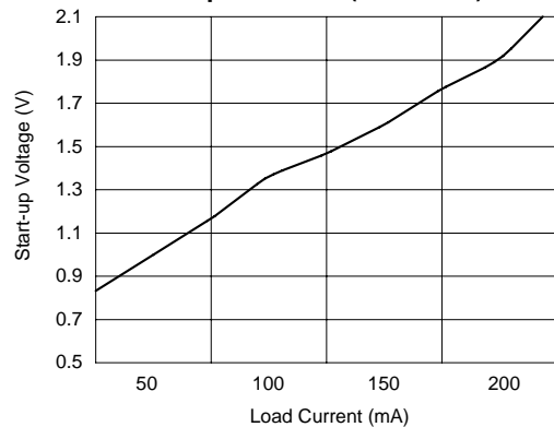
Start-up Input Voltage vs Output current (PWM Mode)
