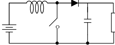
Figure 3: Basic Boost Circuit
