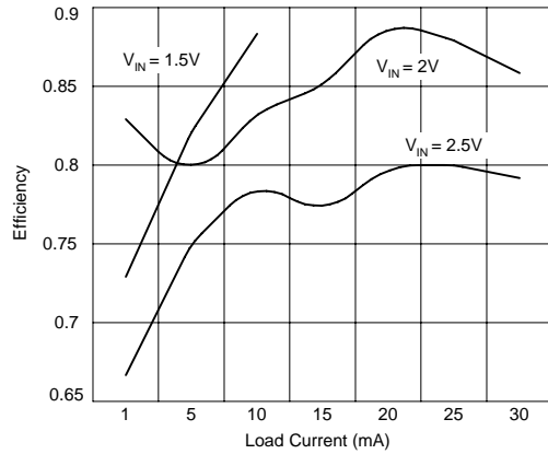
Efficiency (PFM Mode)
