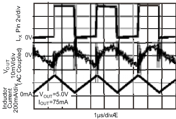
Load Switching Waveforms (PWM Mode)
