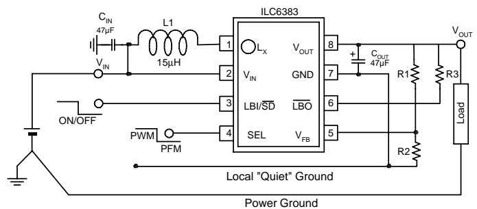
Recommended application circuit schematic for ILC6383CIR-ADJ
