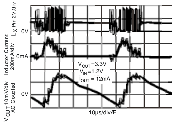
Load Switching Waveforms (PFM Mode)
