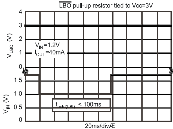
Low Battery Output ( V_{IN} < V_{TH} for Less than 100ms)
