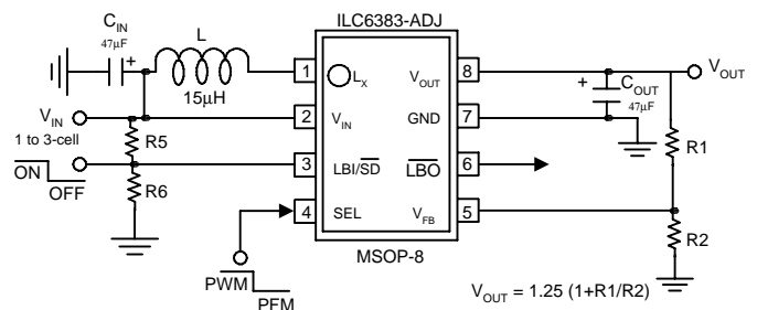
Figure 2: ILC6383CIR-ADJ
