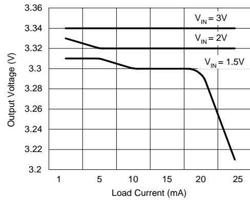
Load Regulation (PFM Mode)
