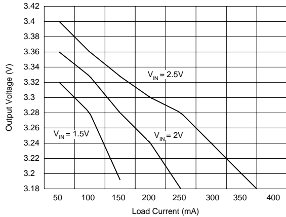
Load Regulation (PWM Mode)
