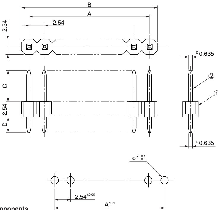
PCB layout for reference only
