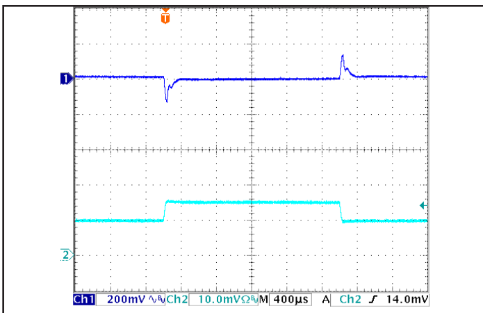
Figure 5: Output voltage response to step-change in load current (50%-75%-50% of I out (max); dI/dt = 0.1 A/µs). Load cap: 100 µF electrolytic cap and 1 µF ceramic cap. Ch 1: V out (200 mV/div), Ch 2: I out (5 A/div).
