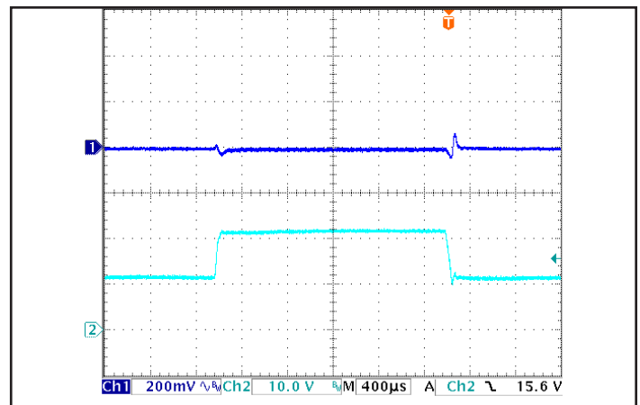
Figure 6: Output voltage response to step-change in input voltage (250 V/ms). Load cap: 100 µF, electrolytic output capacitance. Ch 1: V out (200 mV/div), Ch 2: V in (10 V/div).
