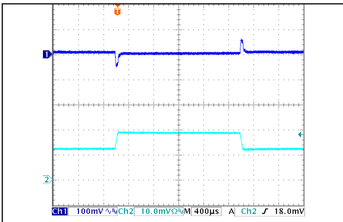
Figure 5: Output voltage response to step-change in load current (50%-75%-50% of I out (max); dI/dt = 0.1 A/µs). Load cap: 100 µF electrolytic cap and 1 µF ceramic cap. Ch 1: V out (100 mV/div), Ch 2: I out (10 A/div).
