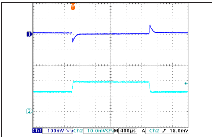
Figure 5: Output voltage response to step-change in load current (50%-75%-50% of I out (max); dl/dt = 0.1 A/µs). Load cap: 100 µF electrolytic cap and 1 µF ceramic cap. Ch 1: V out (100 mV/div), Ch 2: I out (10 A/div).
