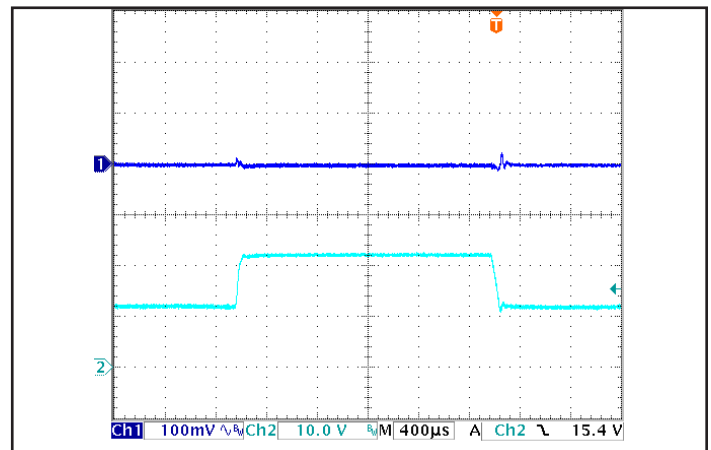
Figure 6: Output voltage response to step-change in input voltage (250 V/ms). Load cap: 100 µF, electrolytic output capacitance. Ch 1: V out (100 mV/div), Ch 2: V in (10 V/div).
