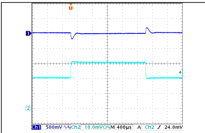
Figure 5: Output voltage response to step-change in load current (50%-75%-50% of I out (max); di/dt = 0.1 A/µs). Load cap: 100 µF electrolytic cap and 1 µF ceramic cap. Ch 1: V out (500 mV/div), Ch 2: I out (1 A/div).
