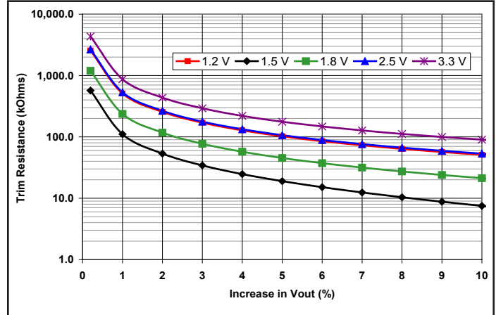
Common Figure 2: Trim graph for trim-up 1.2 to 3.3V outputs.
