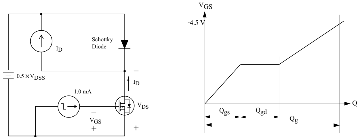
Fig. 1 Gate Charge
