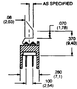
Cross Sectional View
