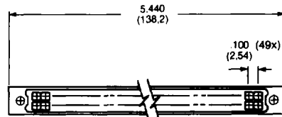
Mating Blade View
