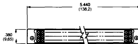
Mating Blade View
