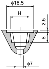
Detail "A" (Press. conn.)
