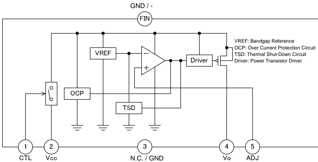
Figure 3. Block Diagram
