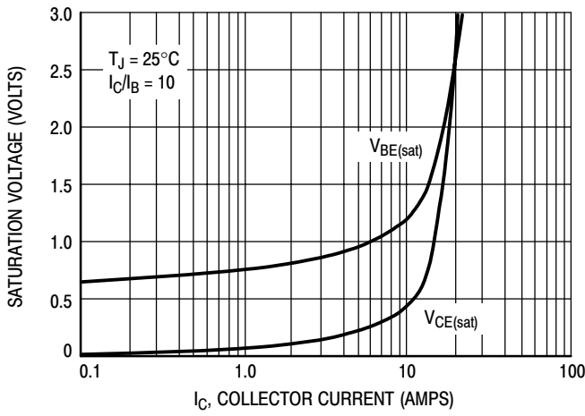
Figure 7. Typical Saturation Voltages
