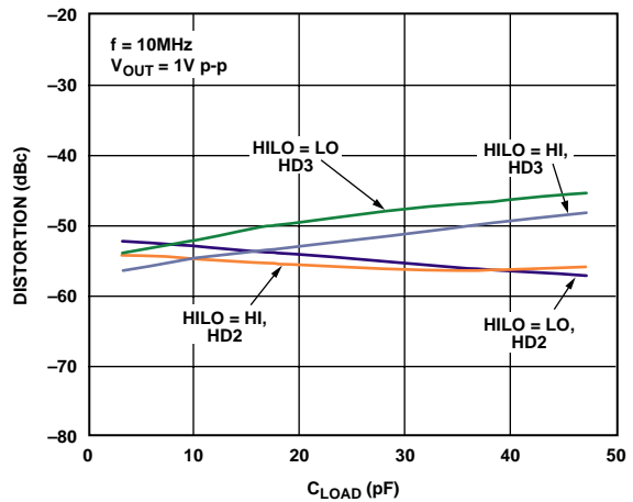
Figure 26. Harmonic Distortion vs. C_{LOAD} (See Figure 53)
