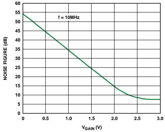
Figure 24. Noise Figure vs. V_{GAIN} for R_S = R_{IN} = 50\ \Omega
