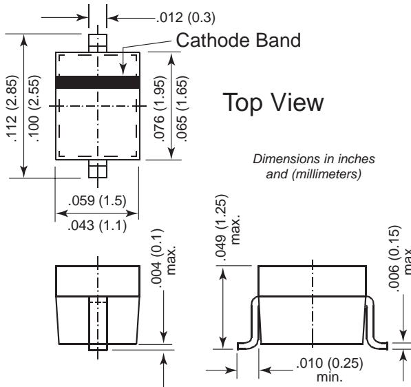
SOD-323
