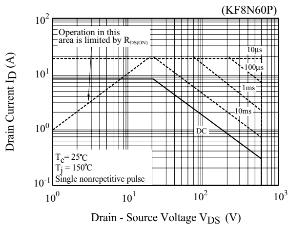
Fig9. Safe Operation Area (KF8N60P)
