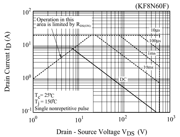
Fig10. Safe Operation Area (KF8N60F)
