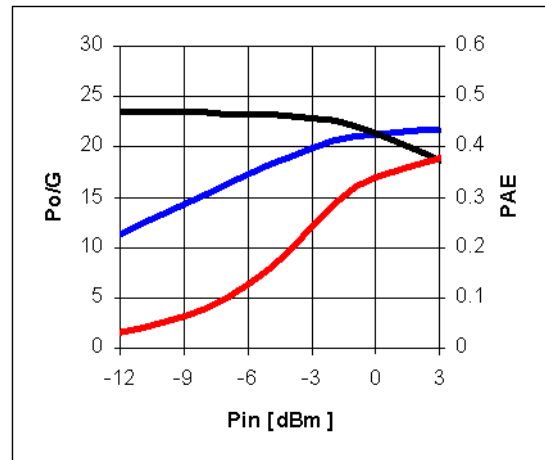
500 MHz, 5V/86mA
