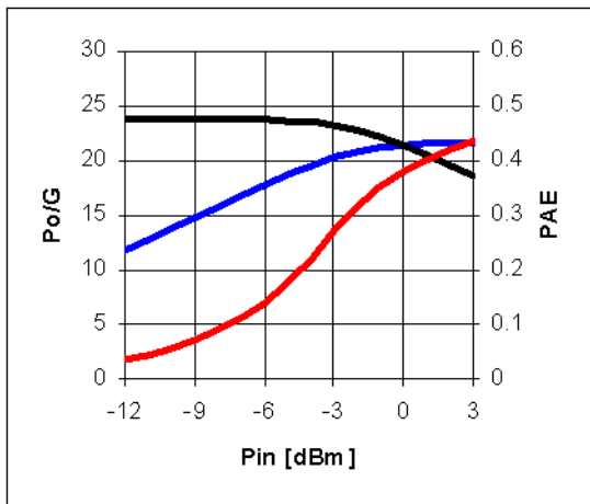
200MHz, 5V/86mA
