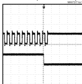
HIGH-SPEED TO LOW-SPEED TRANSITION (EXPANDED SCALE)
