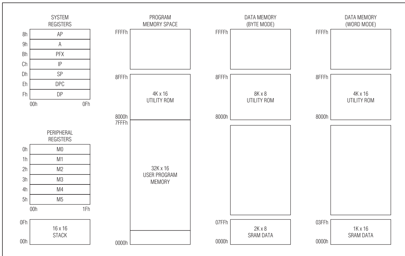
Figure 6. Memory Map
