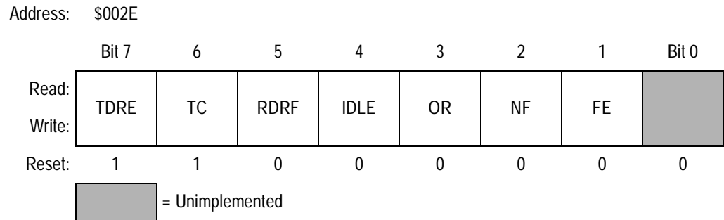
Figure 7-7. Serial Communications Status Register (SCSR)
