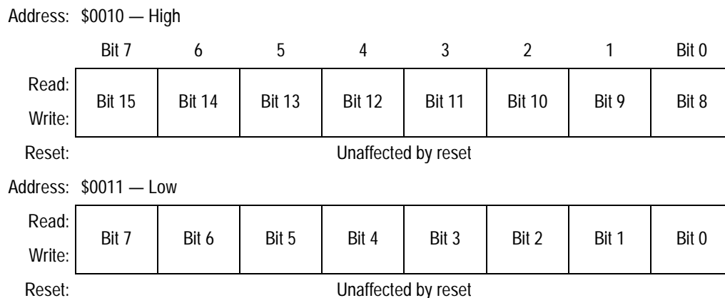
Figure 9-6. Timer Input Capture Register 1 (TIC1)
