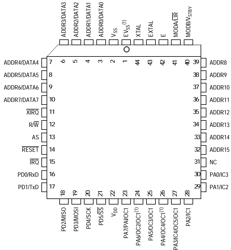
Figure 2-1. Pin Assignments for 44-Pin PLCC
