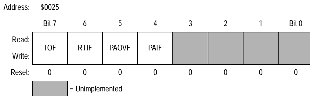
Figure 9-19. Timer Interrupt Flag 2 Register (TFLG2)
