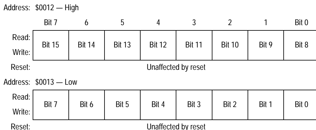
Figure 9-7. Timer Input Capture Register 2 (TIC2)
