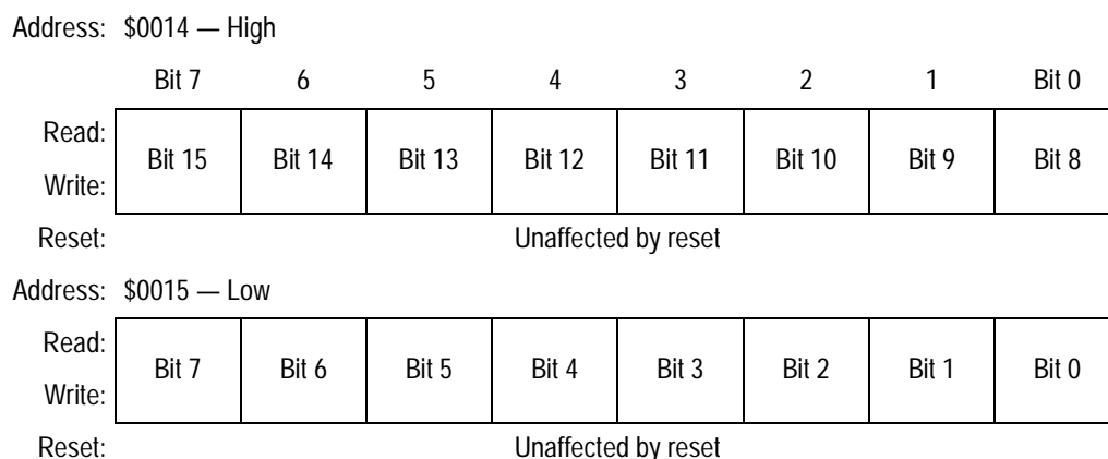
Figure 9-8. Timer Input Capture Register 3 (TIC3)
