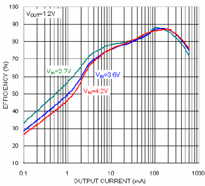
Fig. 4: Efficiency vs Output Current (mA)
