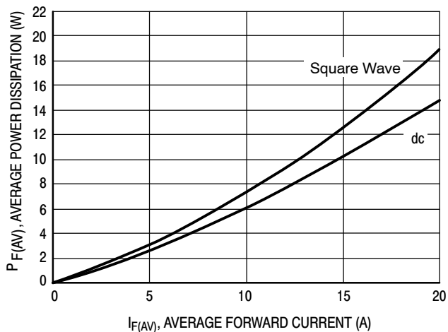
Figure 8. Forward Power Dissipation
