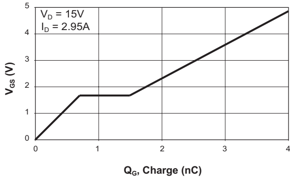
Gate Charge
