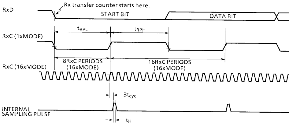
Figure 6.3 Receiver Clock and Data
