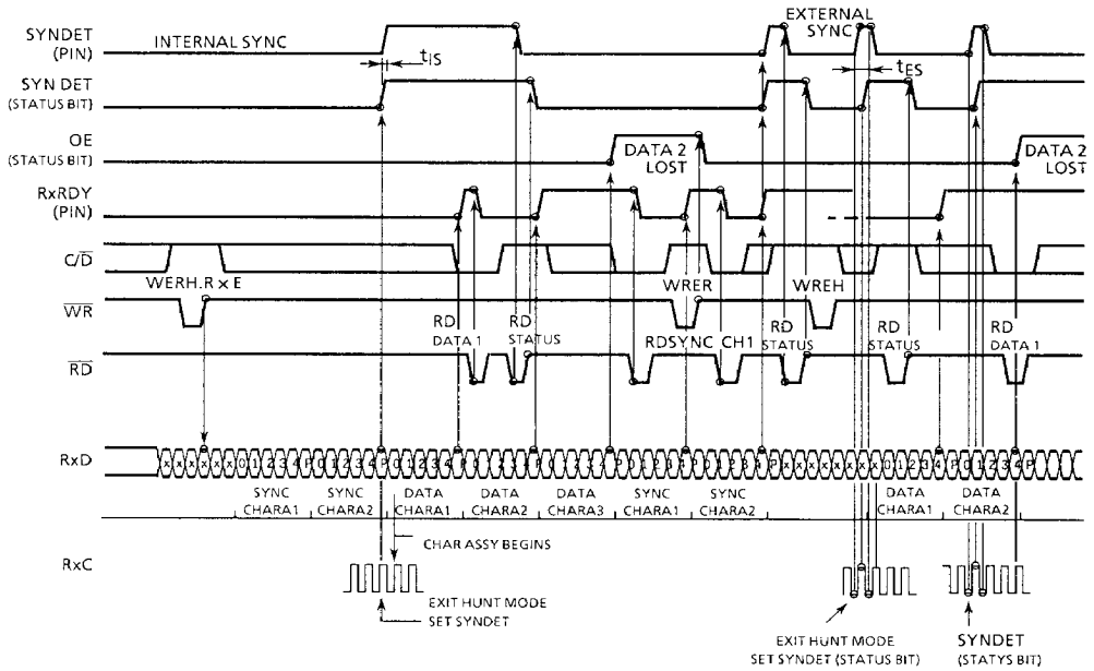
Figure 6.9 Receiver Control and Flag Timing (SYNC Mode)
