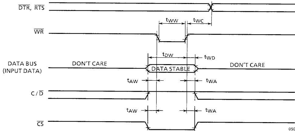
Figure 6.6 Write Control or Output Port Cycle (MPU→8251A)
