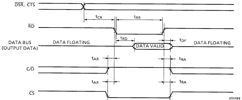
Figure 6.7 Read Control or Input Port Cycle (8251A→MPU)
