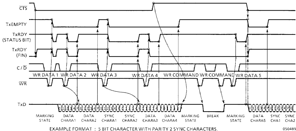
Figure 6.8 Transmitter Control and Flag Timing (SYNC Mode)
