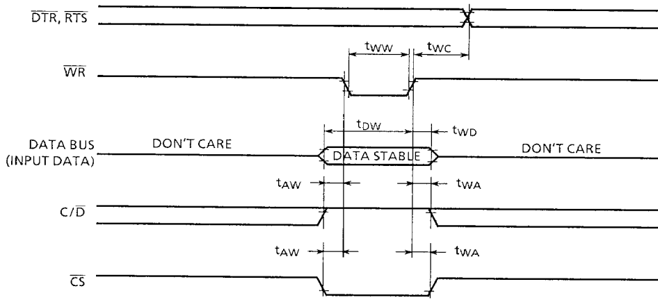
Figure 6.6 Write Control or Output Port Cycle (MPU → 82C51A)
