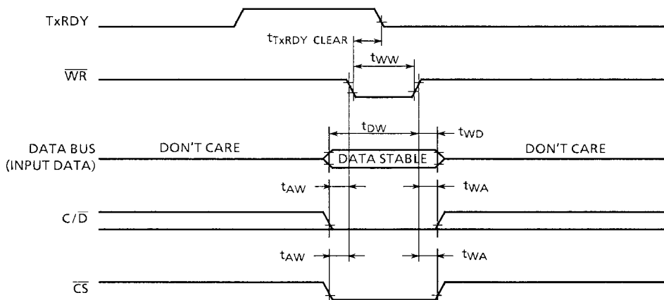
Figure 6.4 Write Data Cycle (MPU → 82C51A)
