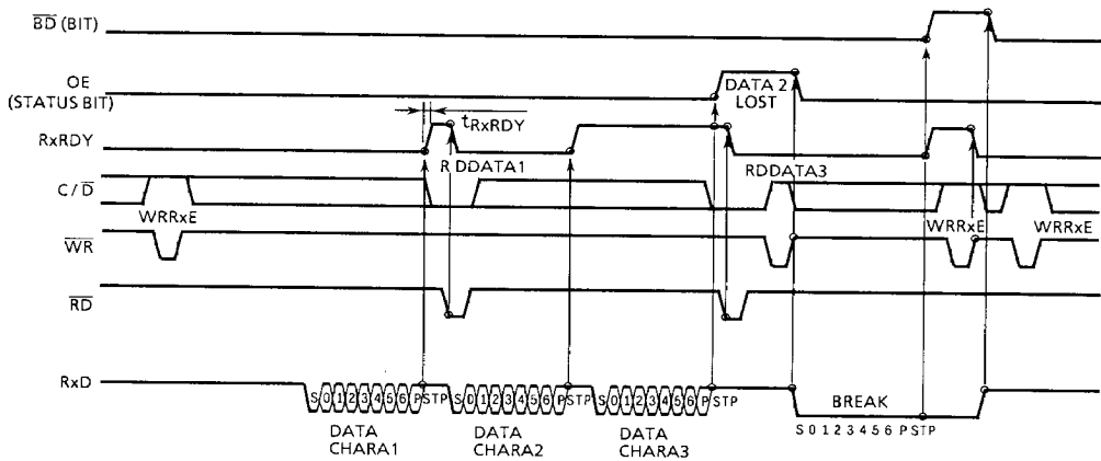
Figure 6.11 Receiver Control and Flag Timing (ASYNC Mode)
