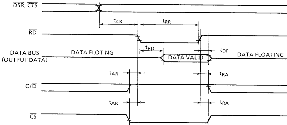
Figure 6.7 Read Control or Input Port Cycle (82C51A → MPU)
