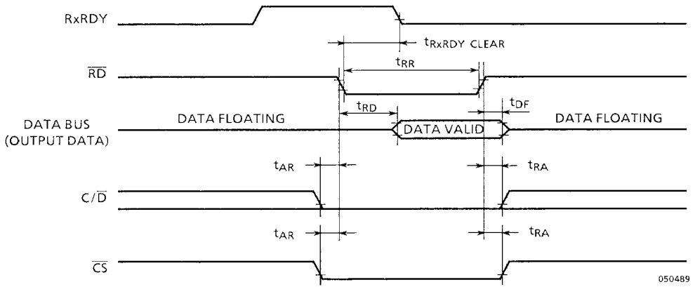
Figure 6.5 Read Data Cycle (8251A→MPU)
