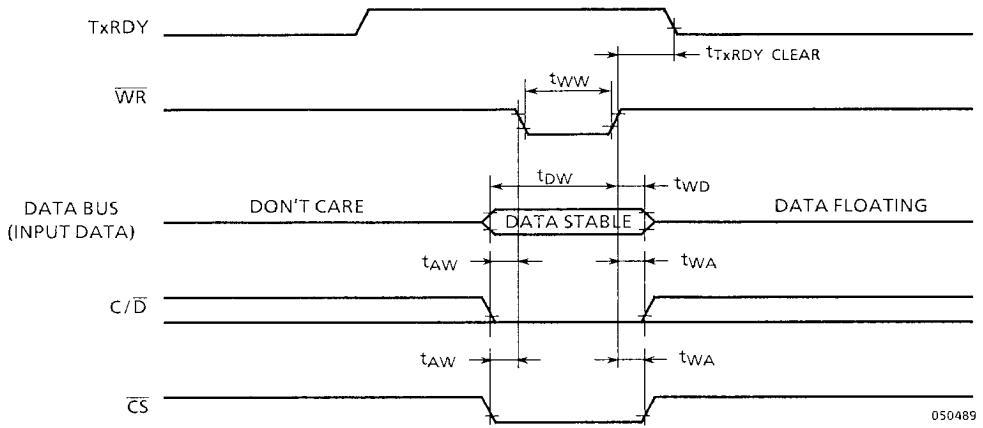
Figure 6.4 Write Data Cycle (MPU→8251A)
