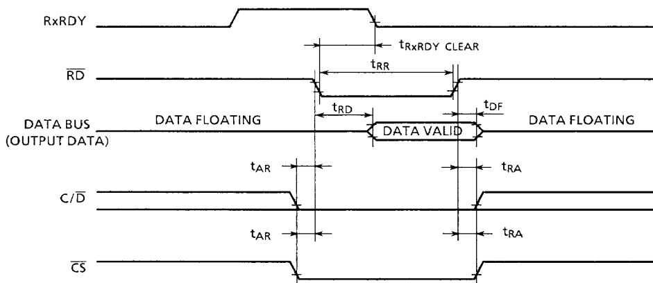
Figure 6.5 Read Data Cycle (82C51A → MPU)
