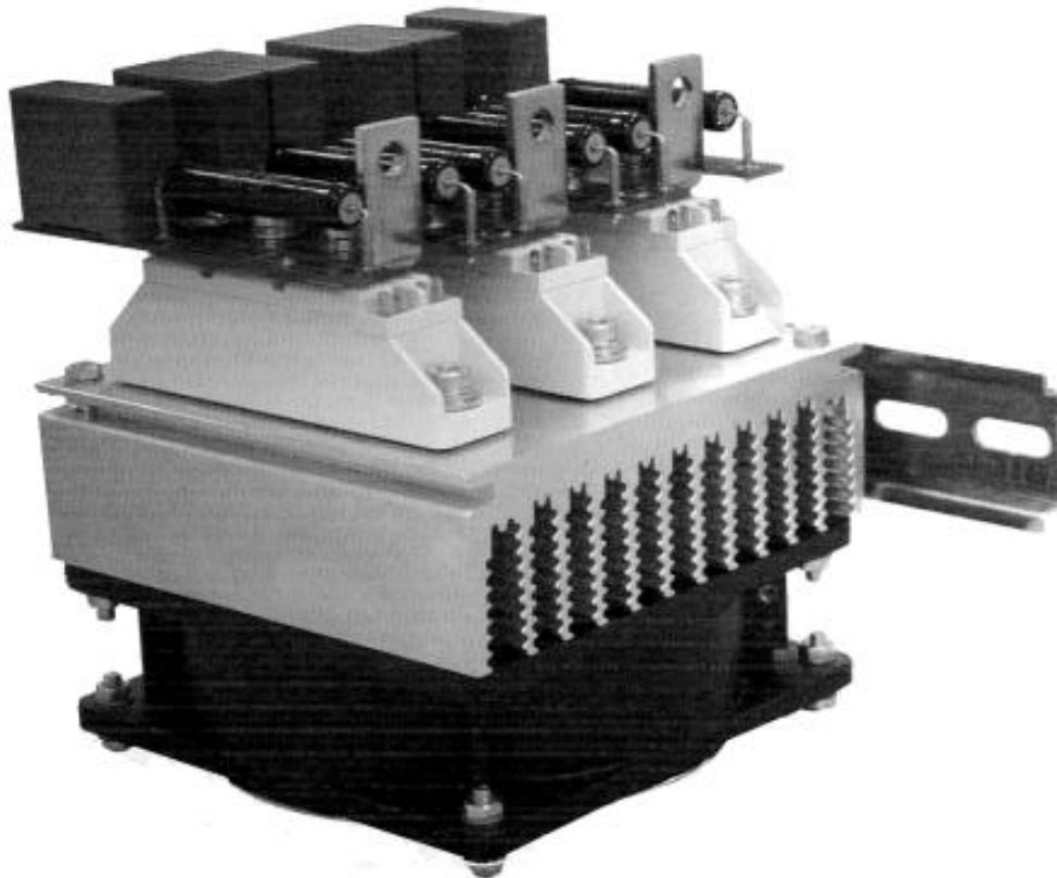
1.Application example using P x120, fan SKF 3 and 3x SEMIPACK 1 modules to give a three phase bridge rectifier
