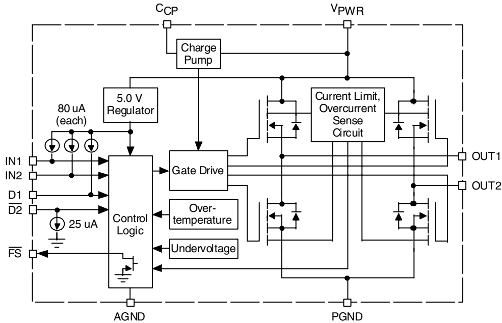
Figure 1. PC33886 Internal Block Diagram
