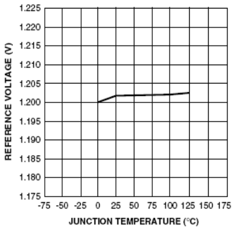
Figure 3. Reference Voltage vs. Temperature
