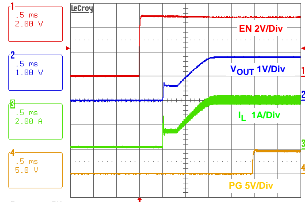
FIGURE 38. SOFT-START AT FULL LOAD
