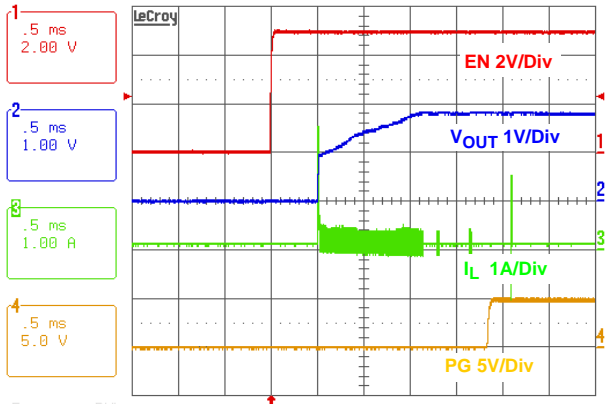
FIGURE 37. SOFT-START AT NO LOAD (PFM)
