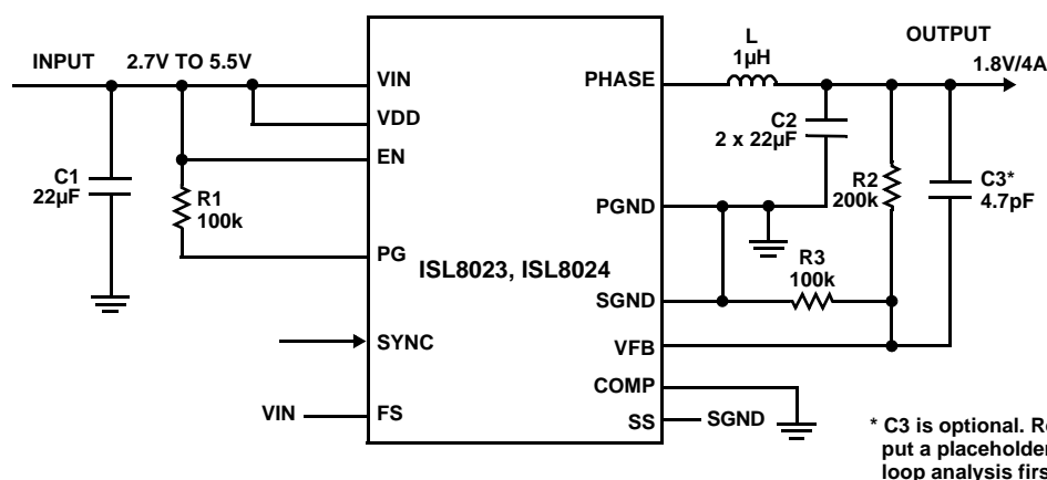
FIGURE 3. TYPICAL APPLICATION DIAGRAM
