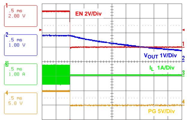
FIGURE 26. SOFT-DISCHARGE SHUTDOWN
