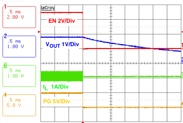
FIGURE 39. SOFT-DISCHARGE SHUTDOWN
