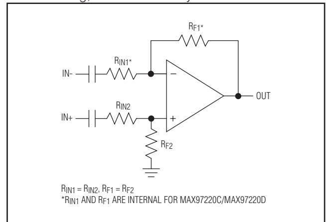
Figure 2. Differential Input Configuration
