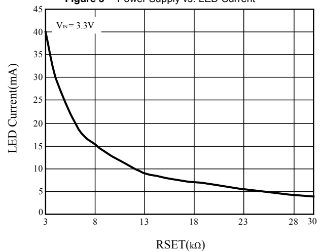
Figure 5 R SET vs. LED Current
