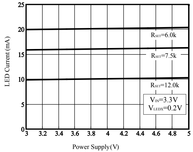
Figure 3 Power Supply vs. LED Current
