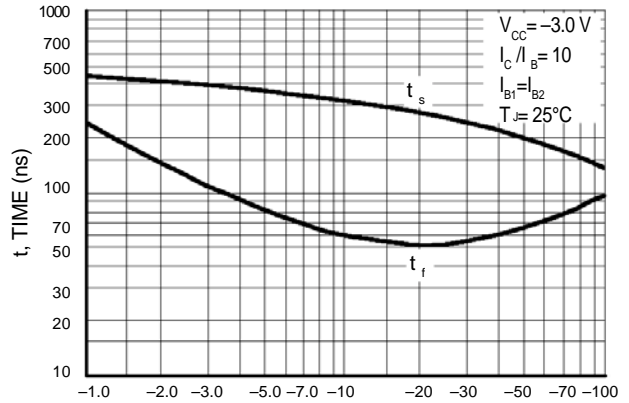
Figure 11. Turn-Off Time
