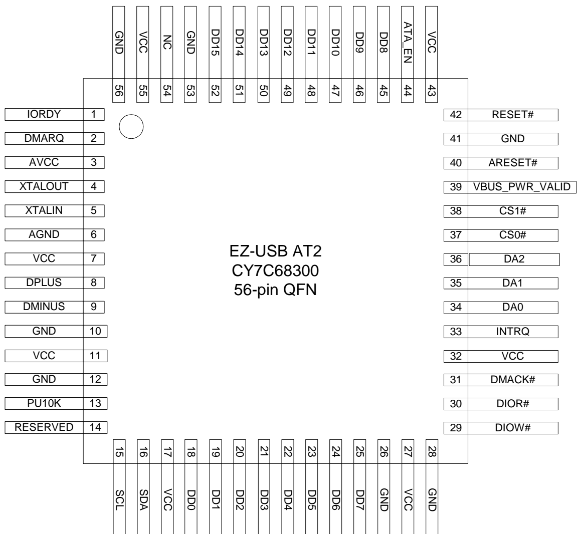
Figure 2-2. 56-pin QFN
