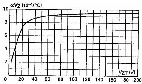
Fig. 3 - Temperature coefficient \alpha V_Z = \frac{\Delta V_{ZT}}{V_{ZT} \Delta T} versus V_{ZT} (typical values).
