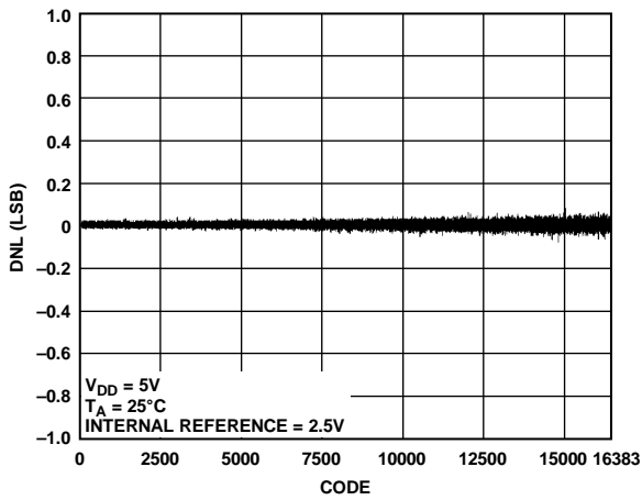
Figure 20. AD5685R DNL
