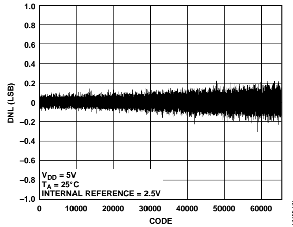
Figure 19. AD5686R DNL
