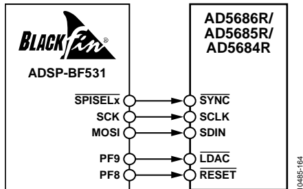
Figure 60. ADSP-BF531 Interface
