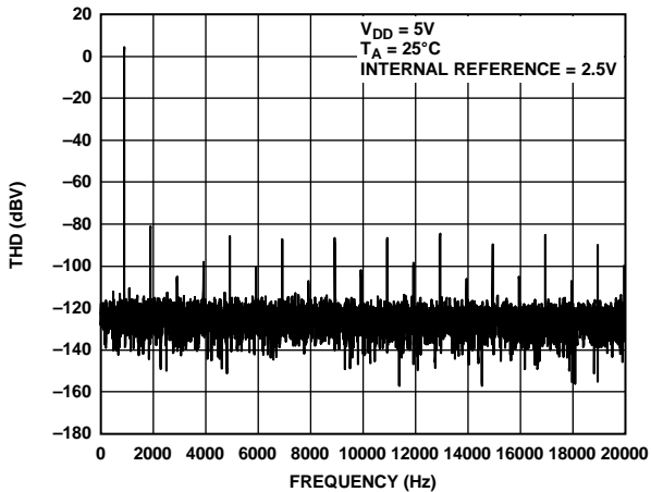
Figure 46. Total Harmonic Distortion @ 1 kHz
