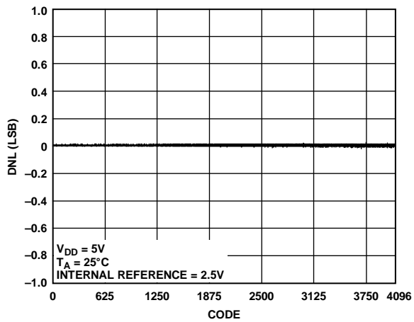
Figure 21. AD5684R DNL
