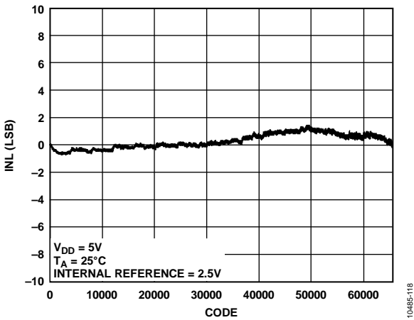
Figure 16. AD5686R INL
