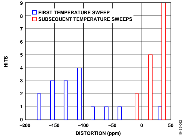
Figure 59. Thermal Hysteresis
