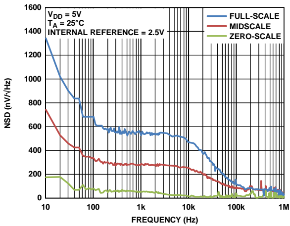
Figure 45. Noise Spectral Density
