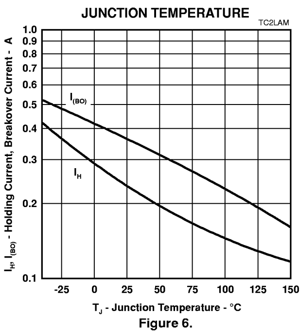
HOLDING CURRENT & BREAKOVER CURRENT VS JUNCTION TEMPERATURE
