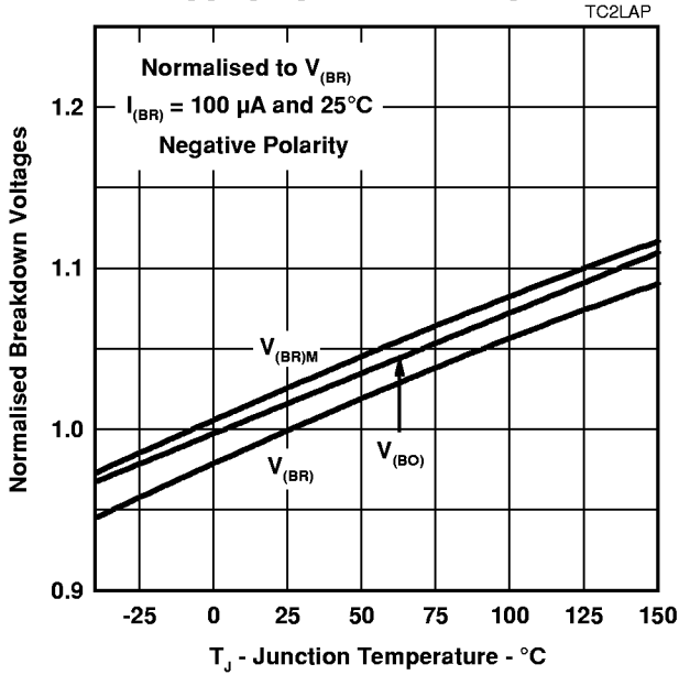
NORMALISED BREAKDOWN VOLTAGES VS JUNCTION TEMPERATURE
