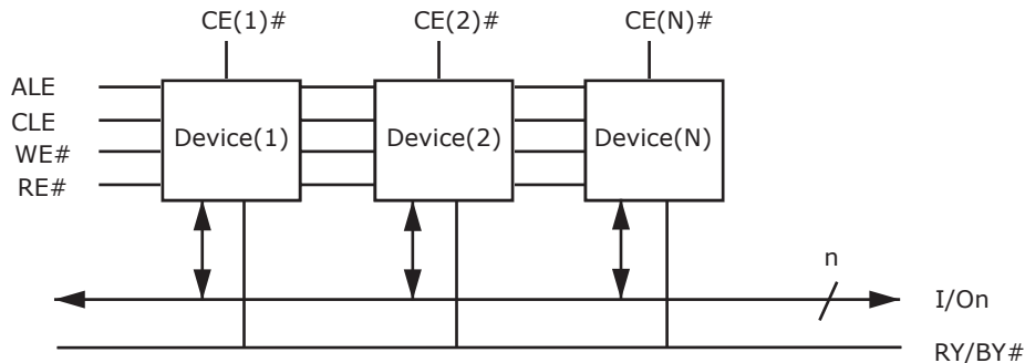
Figure 12.9 Multiple Devices
