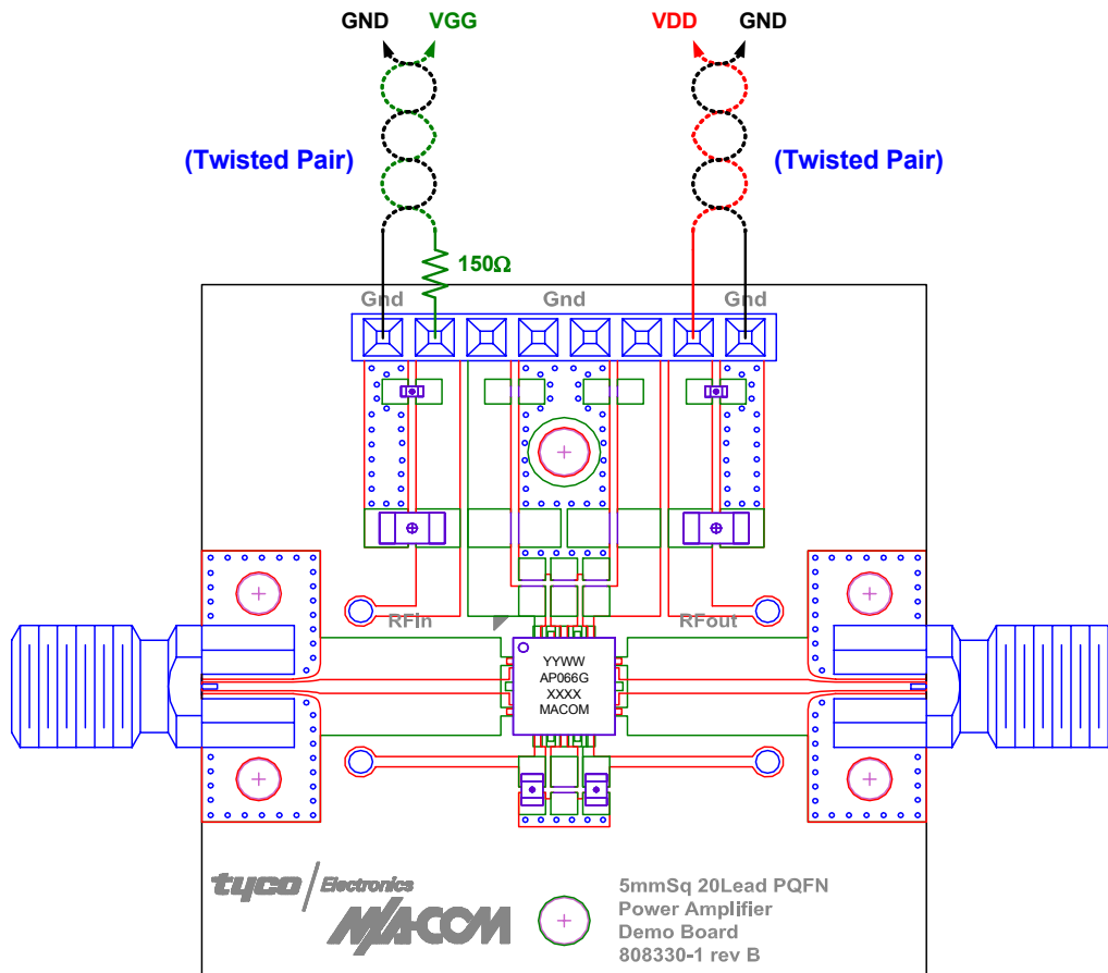
Figure 29. Demonstration Board PN MAAP-000044-SMB003 (available upon request).
