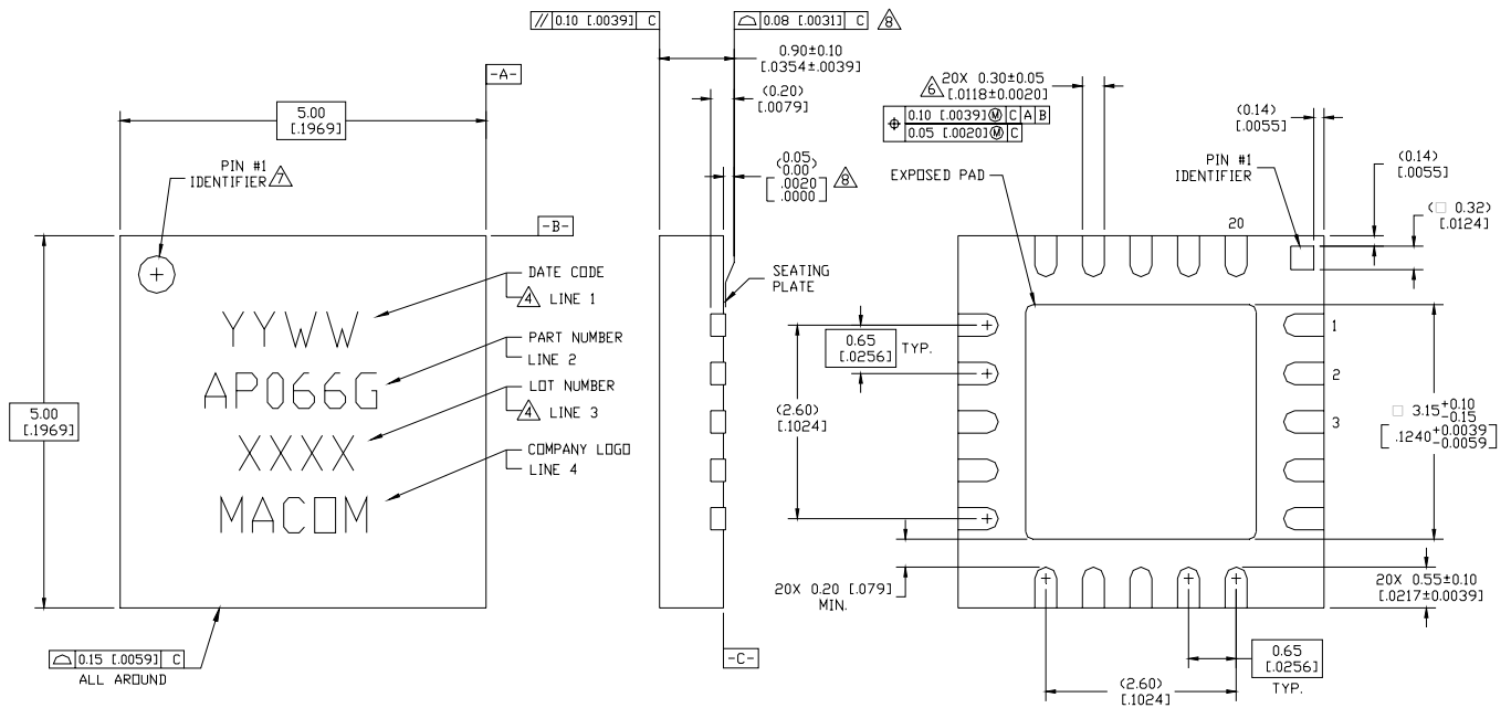
Figure 27. 5x5 mm 20-Lead PQFN.
