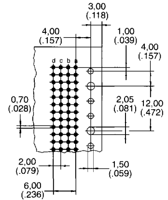
Recommended P.C.B. Hole Pattern, Component Side
