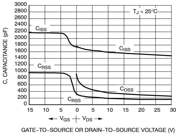
Figure 7. Capacitance Variation
