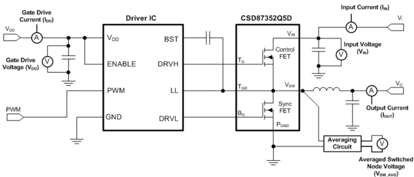
Figure 32. Typical Application
