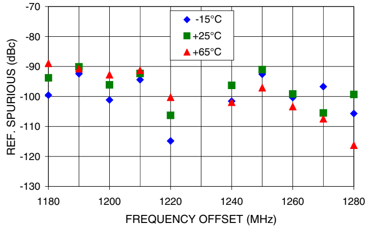
REFERENCE SPURIOUS Vs FREQ. OFFSET @ Fcar = 1230MHz
