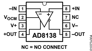
Figure 4. Pin Configuration
