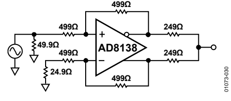
Figure 41. Test Circuit for Output Balance
