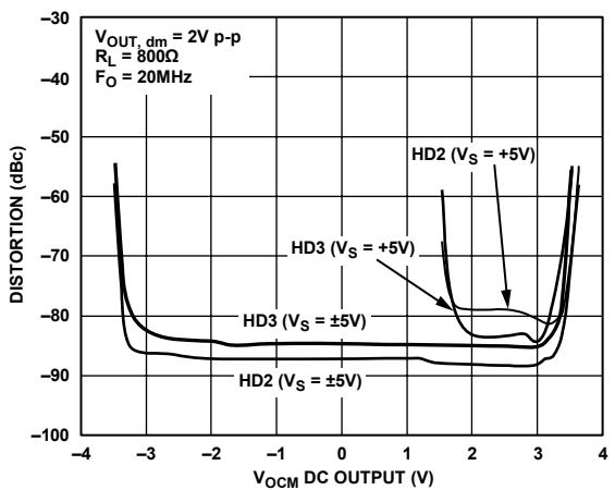
Figure 13. Harmonic Distortion vs. V_{OCM}
