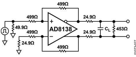
Figure 40. Test Circuit for Cap Load Drive
