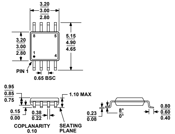
Figure 51. 8-Lead Mini Small Outline Package [MSOP] (RM-8)
