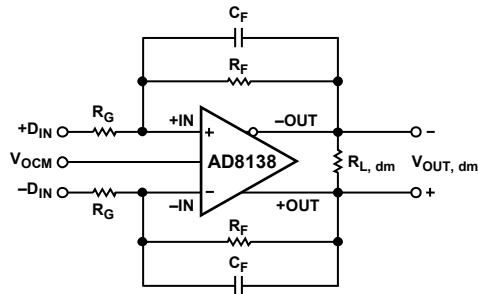
Figure 42. Circuit Definitions
