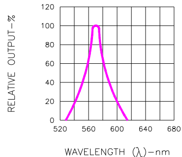
Fig.2 SPECTRAL RESPONSE
