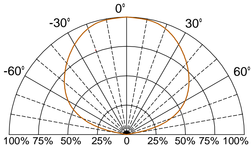
Fig.6 Directivity Radiation
