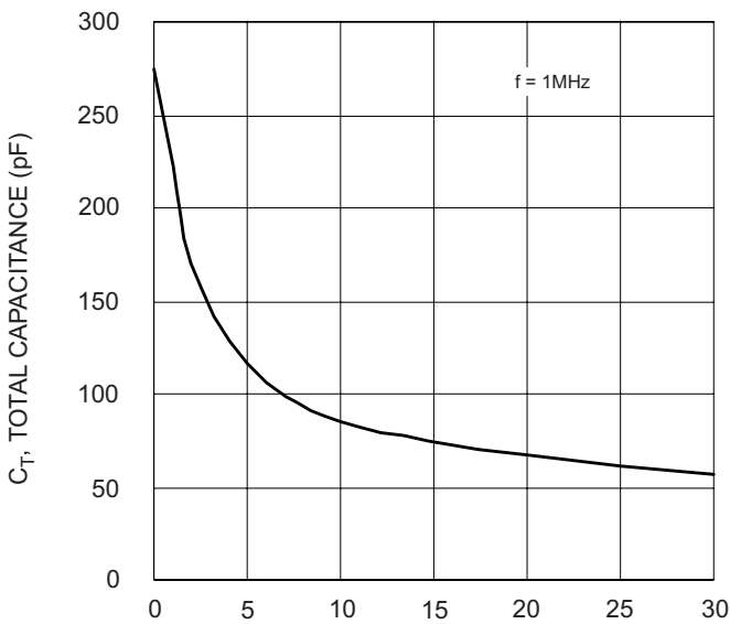
Fig. 3, Typical Total Capacitance
